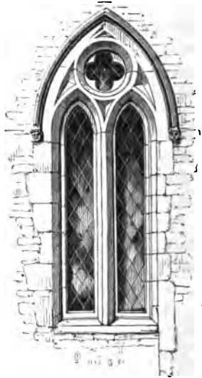
93. Charlton-on-Otmoor, Oxon, c. 1240. Shewing a window of two lights with a quatrefoil in the head of plate-tracery, and a dripstone terminated by the characteristic ornament called a mask or a buckle.
